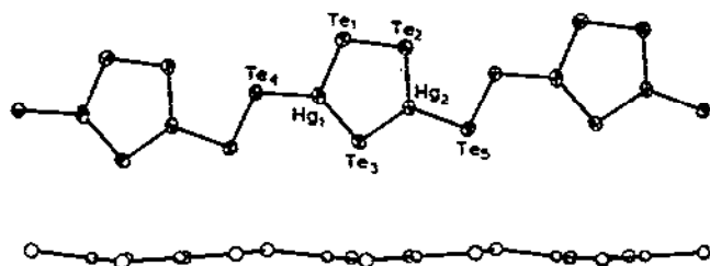
Fig. 35. Two views of the {}^1_{\infty}[\text{Hg}_2\text{Te}_5]^{2-} chain [105].
