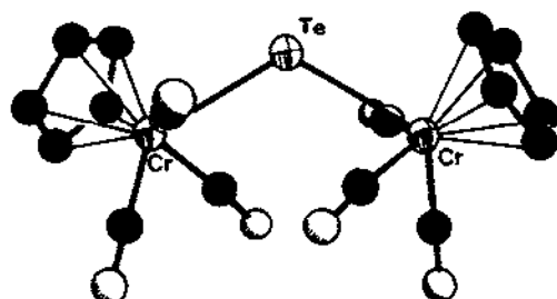
Fig. 9. Structure of the (\eta^5-C_5H_5)_2Cr_2(CO)_6(\mu-Te) molecule [77].
