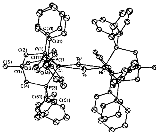
Fig. 18. Structure of the [(\text{triphos})\text{Ni}]_2(\mu\text{-}\eta^2\text{-Te}_2) molecule [96].
