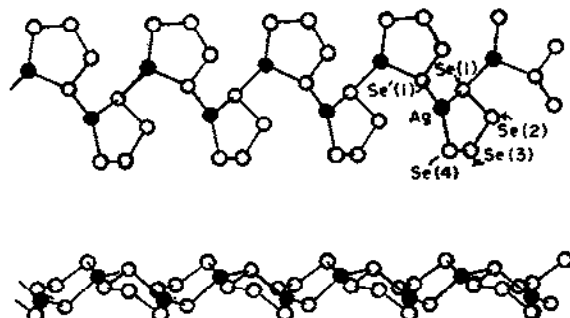
Fig. 34. Two views of the [\text{Ag}(\text{Se}_4)]_n^- chain [134].
