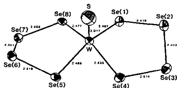
Fig. 32. The \text{WS}(\text{Se}_4)_2^{2-} anion [115].
